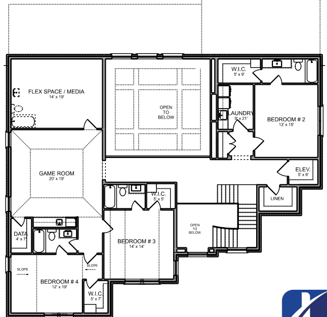
SECOND FLOOR
